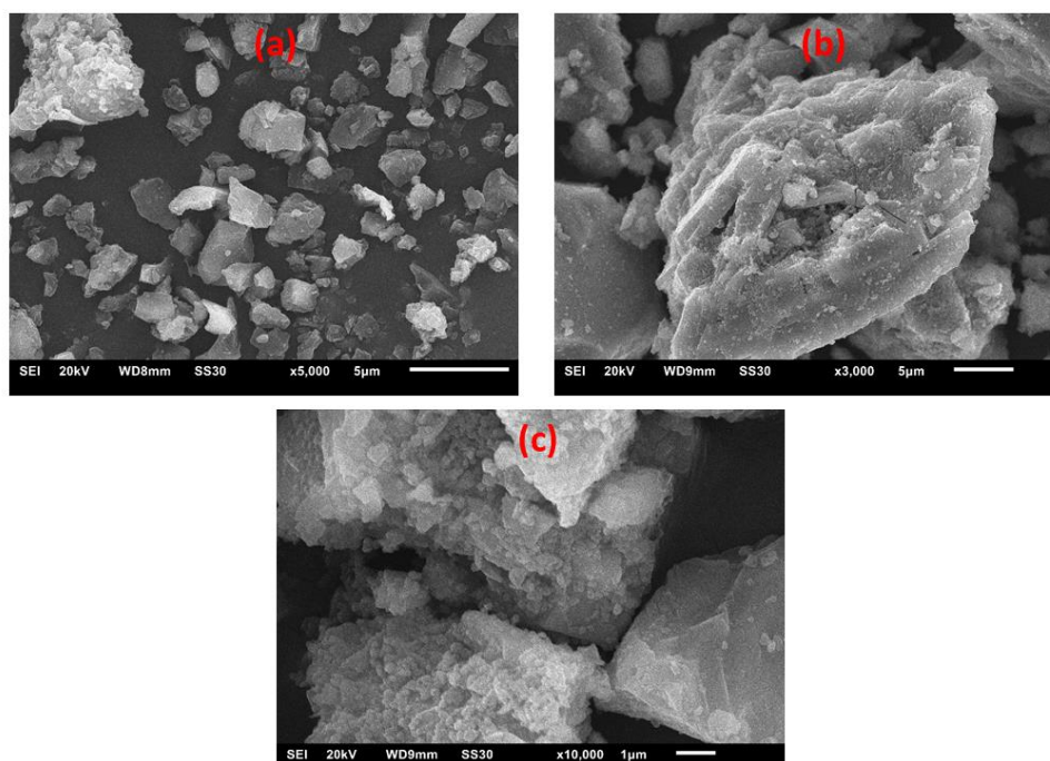
Figure 5: Scanning electron Microscopy of Pz (a), GP 0 (b) and GP 1 (c)
