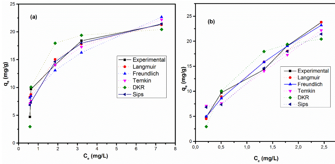
Figure 12: Adsorption isotherm plots for MB onto (a) GP 0 and (b) GP 1 materials
