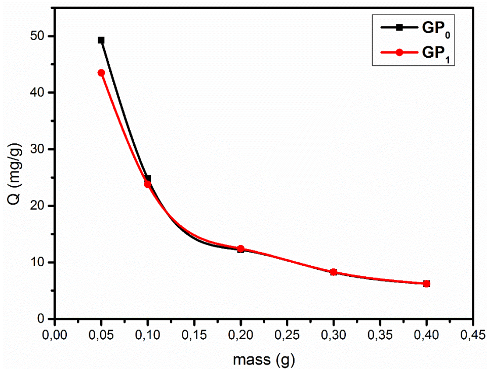
Figure 7: Influence of Adsorbent Dose
