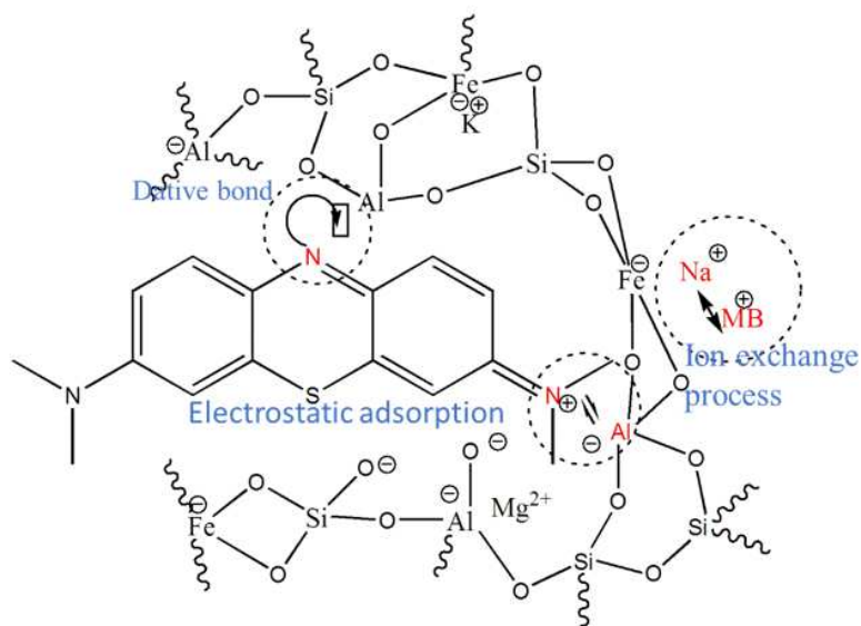
Figure 11: Interaction mechanisms in the GP1-MB system.
