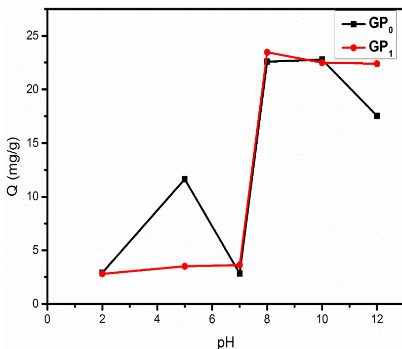
Figure 6: Influence of pH on the adsorption capacity of the different geopolymers.
