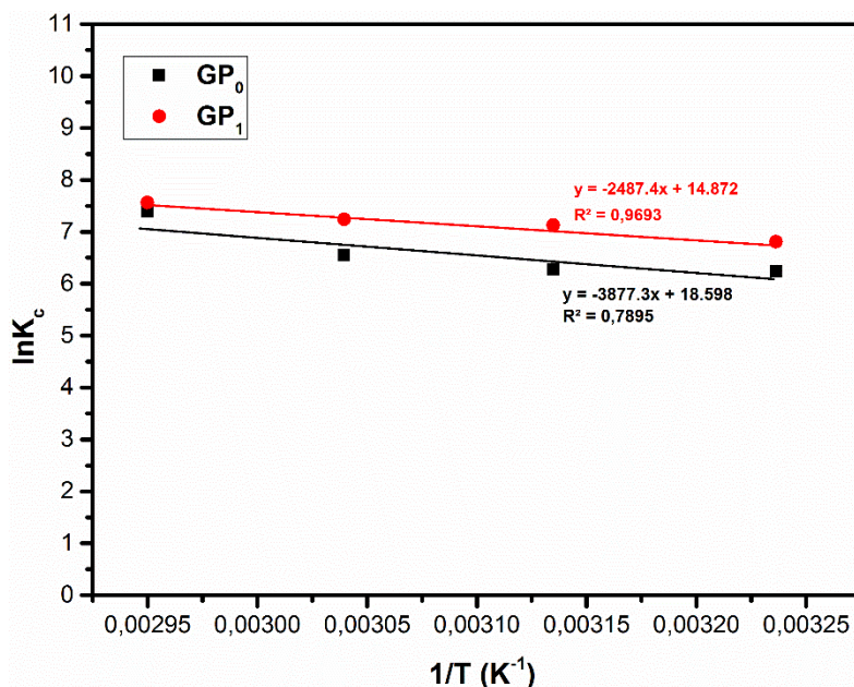
Figure 13: Isotherm plot of van't Hoff.
