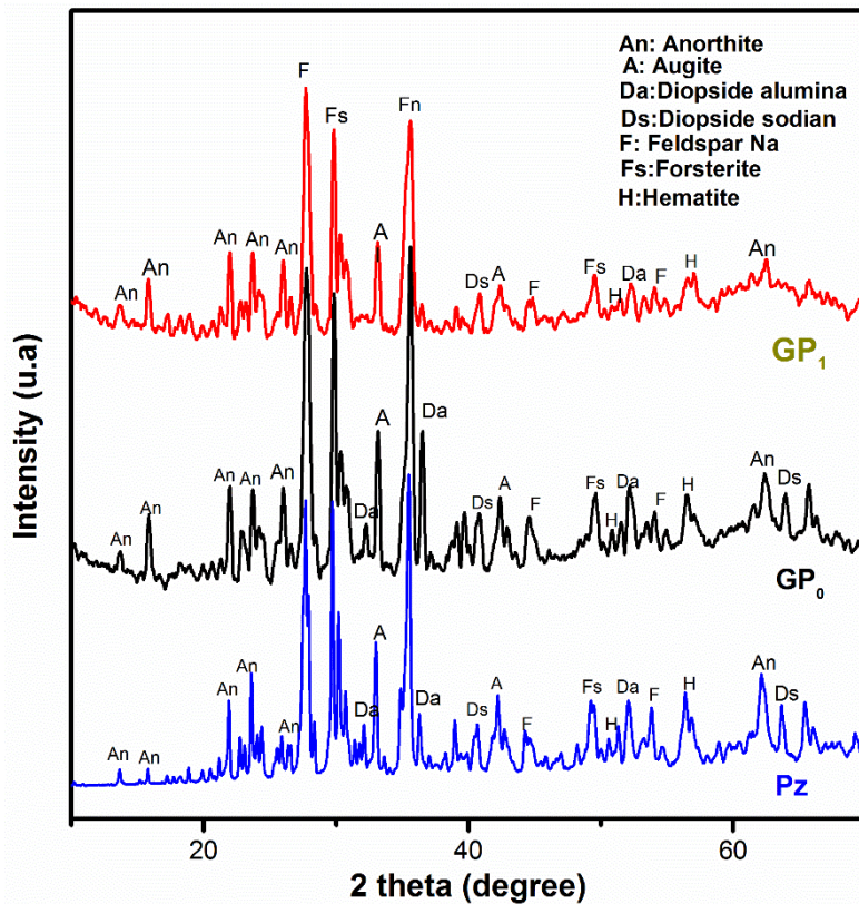
Figure 4: XRD patterns of precursor and GP 0 and GP 1 geopolymer
