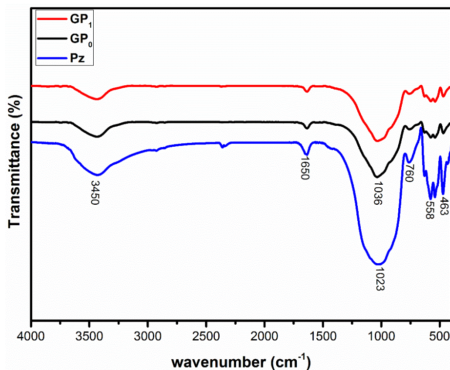
Figure 3: FTIR of the samples Pz, GP 0 and GP 1
