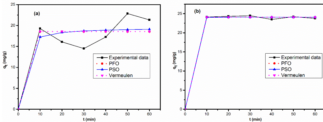
Figure-9: PFO, PSO and Vermeulen models applied to the experimental kinetic data for the adsorption of MB on different geopolymers ((a) GP 0 and (b) GP 1 )
